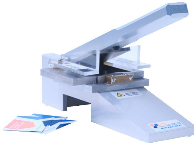
simple cutting process by pushing a lever
